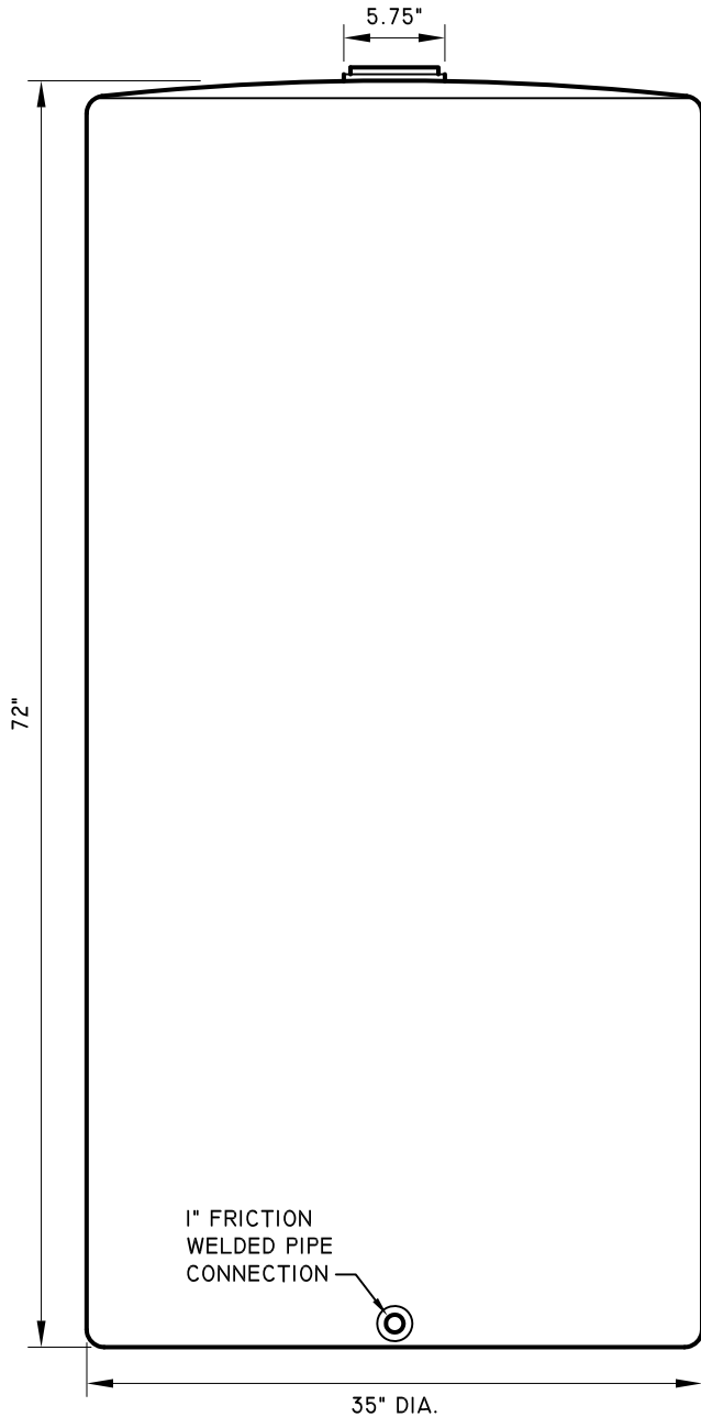
SIDE ELEVATION
