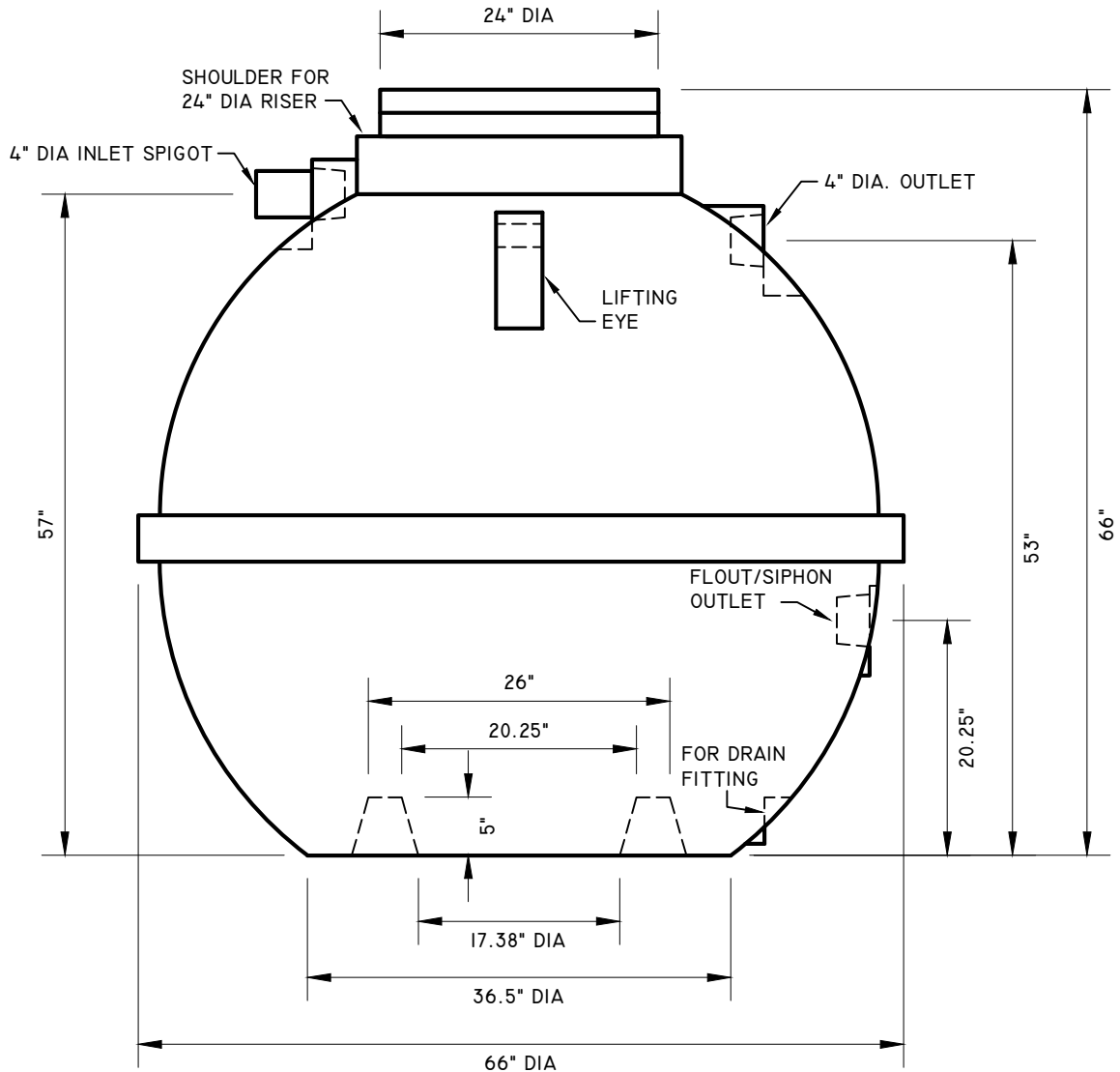
SIDE ELEVATION
