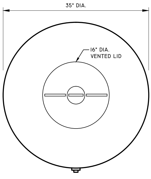
TOP VIEW
