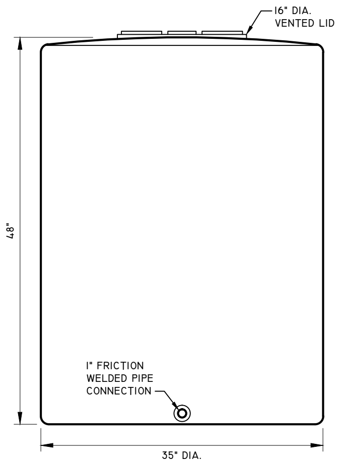
SIDE ELEVATION
