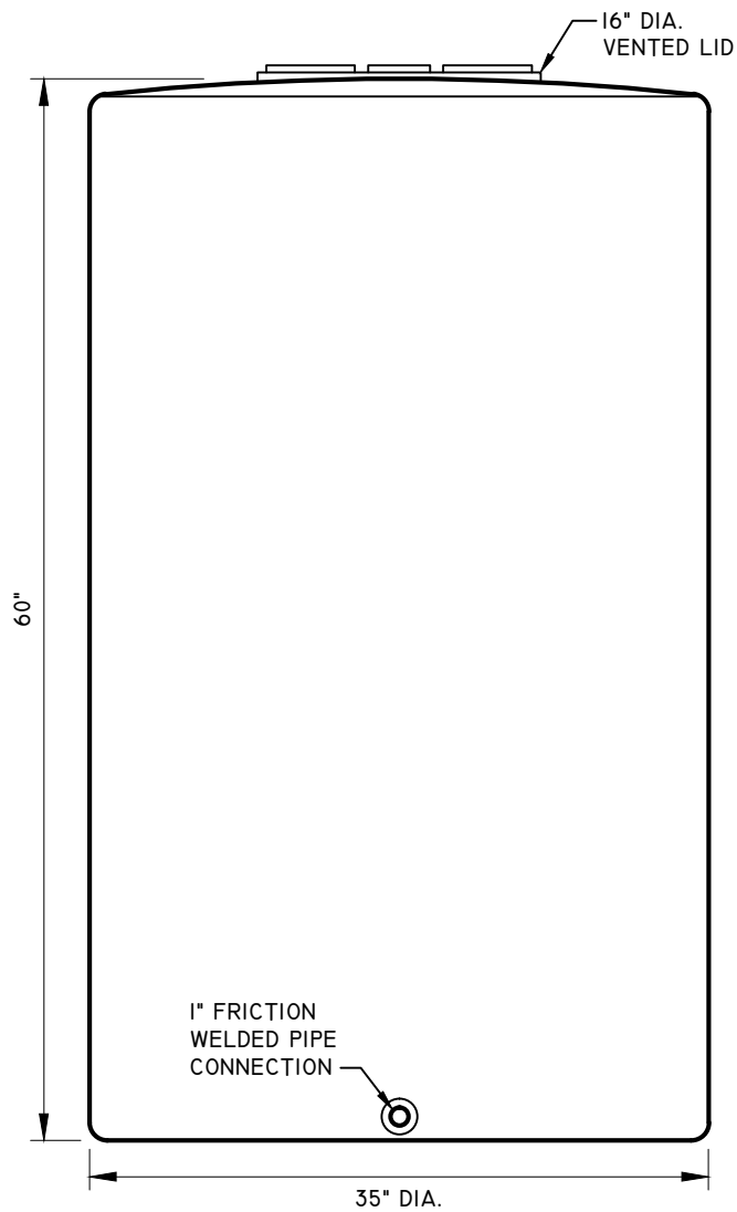
SIDE ELEVATION
