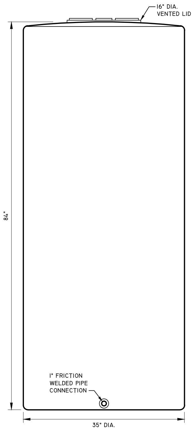
SIDE ELEVATION
