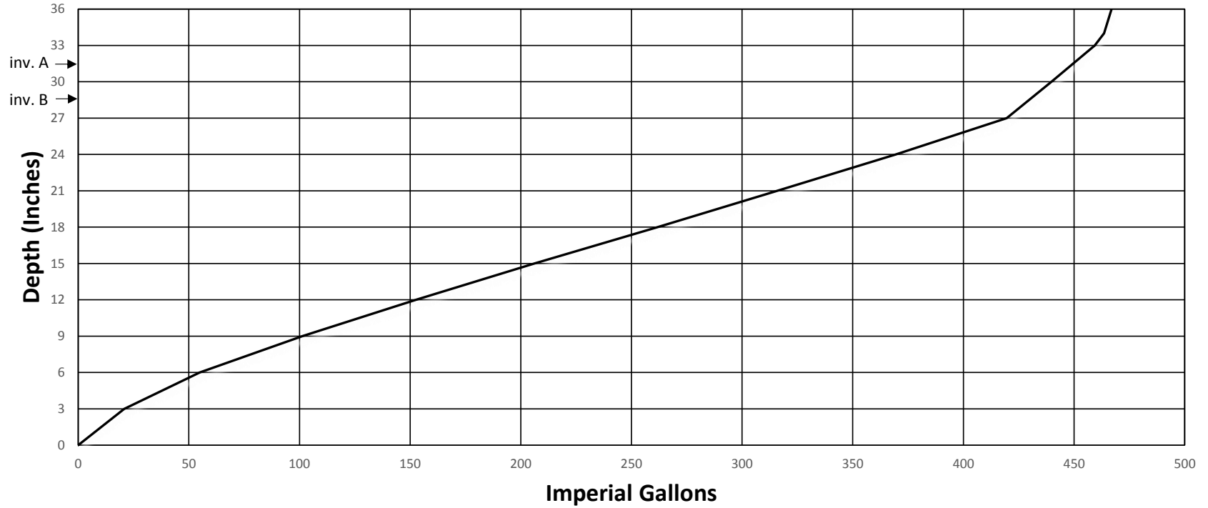
BT 470 BOBBLE TANK (BTU560) - WATER VOLUME PER INCH
